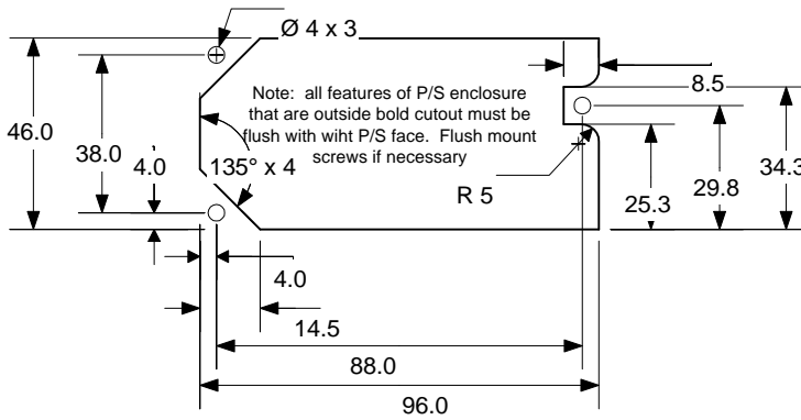
Figure 5 40 mm Profile Mechanical Outline
