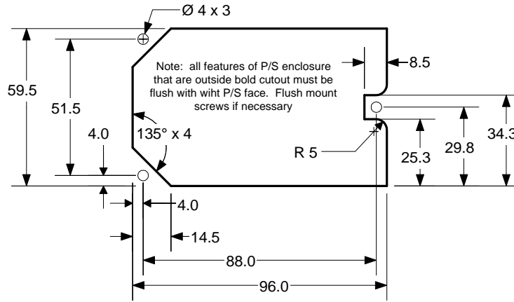
Figure 13 Chassis Cutout
