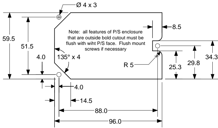
Figure 8 Chassis Cutout
