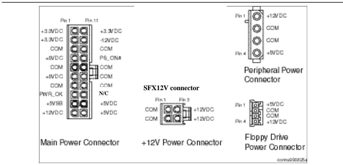
Figure 4. SFX/SFX12V Connectors
