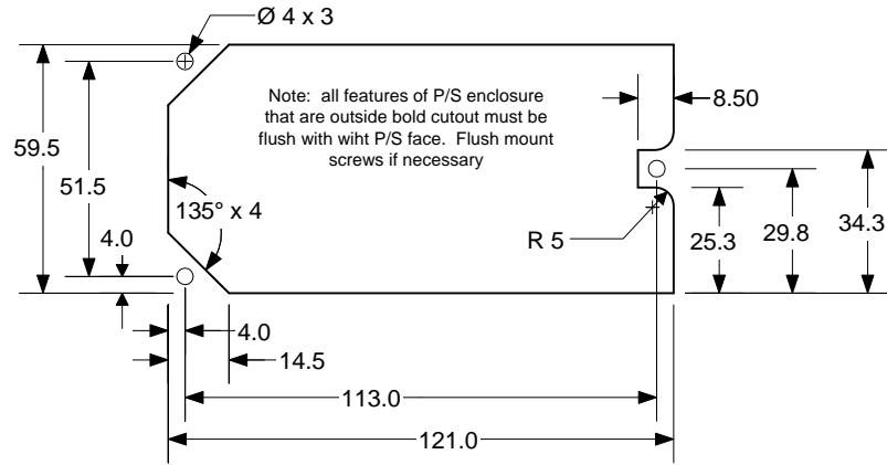
Figure 11 Chassis cutout
