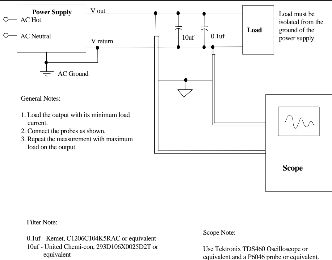
Figure 1. Differential Noise Test Setup
