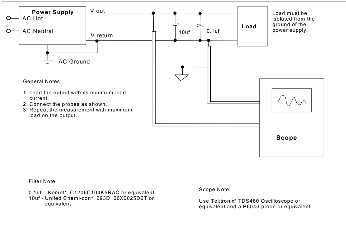
Figure 3. Differential Noise Test Setup
