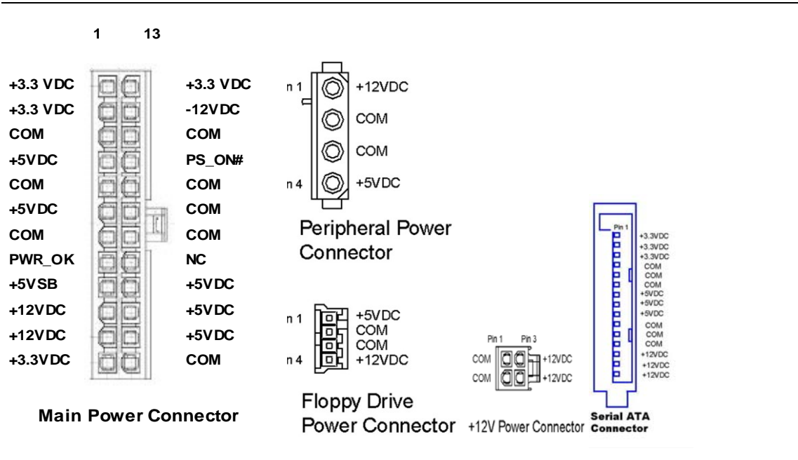
Figure 10. Connectors (Pin-side view, not to scale)
