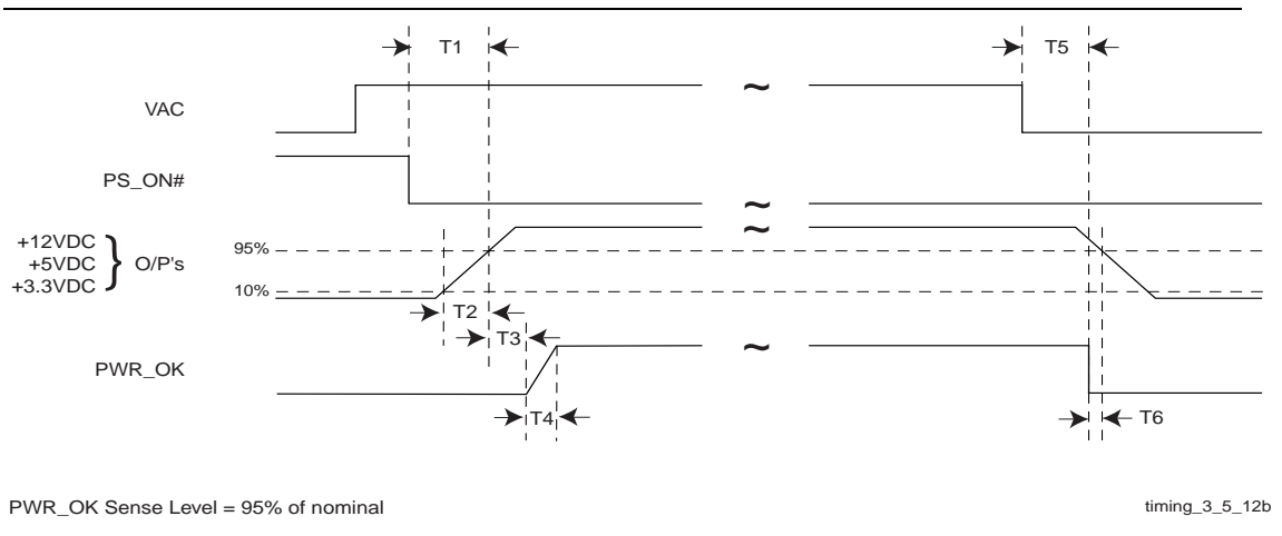
Figure 4. Power Supply Timing
