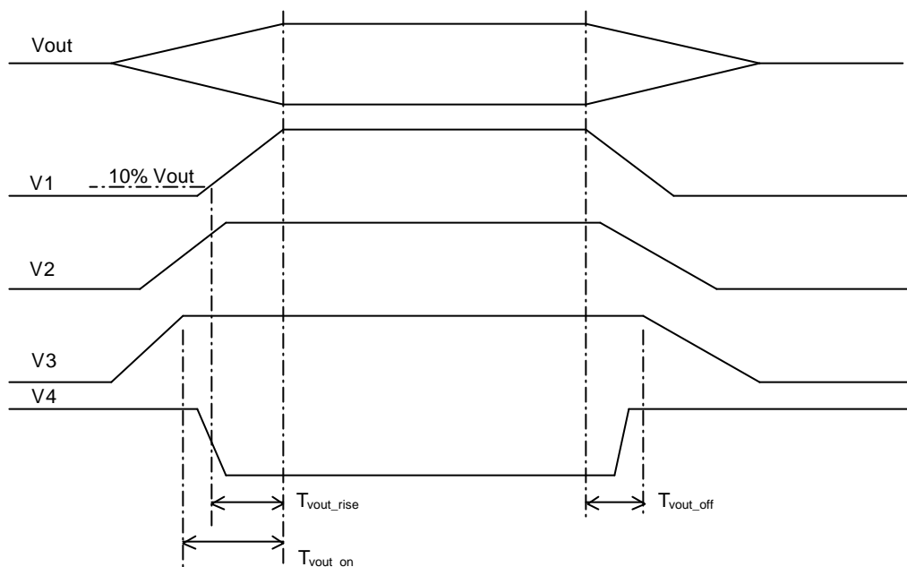
Figure 3: Output Voltage Timing
