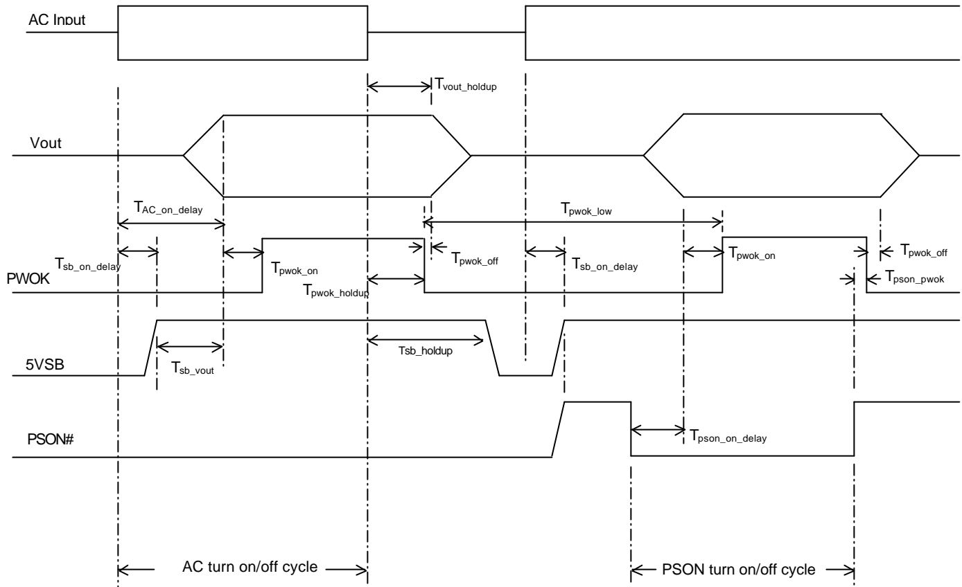
Figure 4: Turn On/Off Timing (Single Power Supply)
