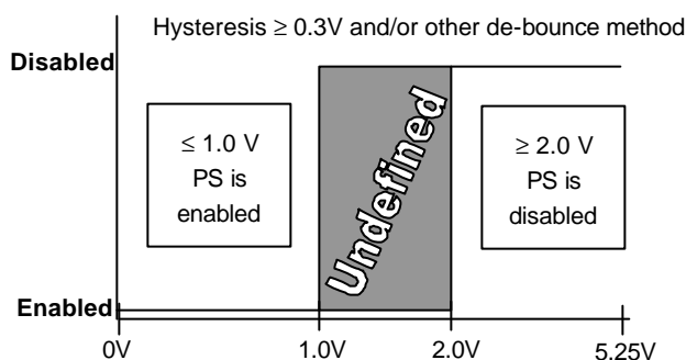
Figure 5: PSON# Signal Characteristics
