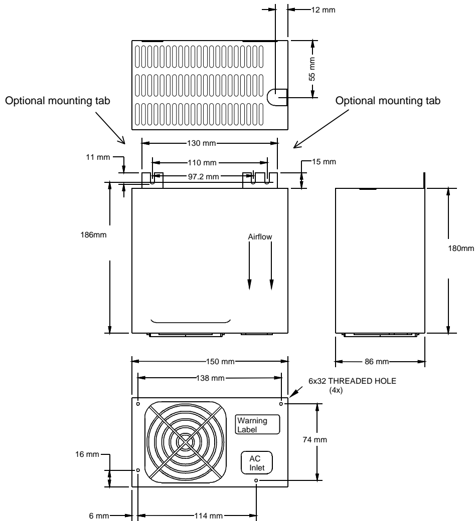
Figure 1: Enclosure Drawing
